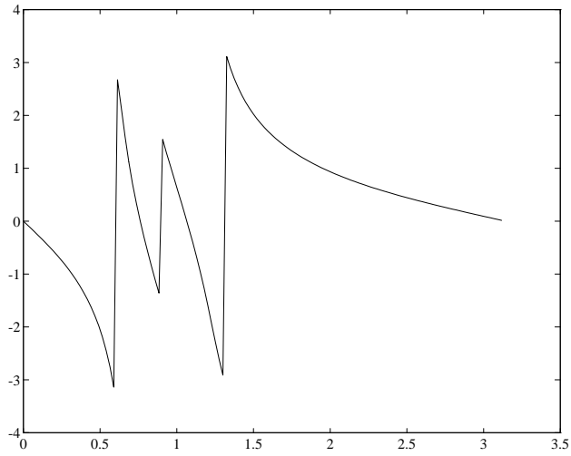
Figure 3: Phase response of the digital filter of Fig. 2.
