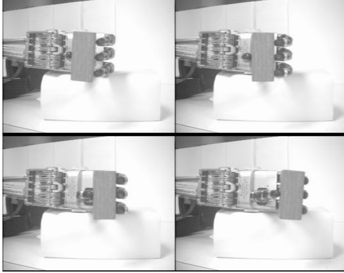
Figure 3: Translation along the x axis
