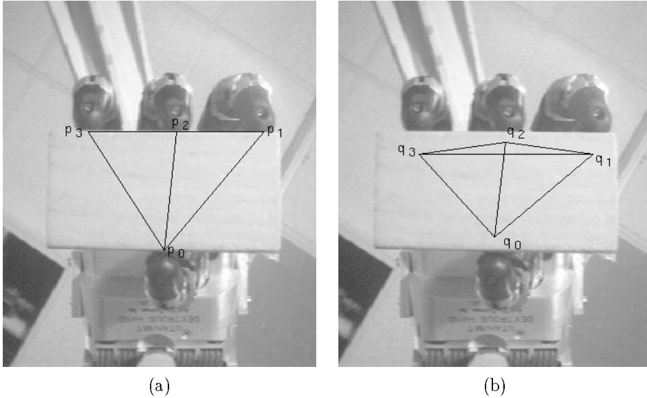
Figure 1: The contact tetrahedron (a) and the grasp tetrahedron (b).
