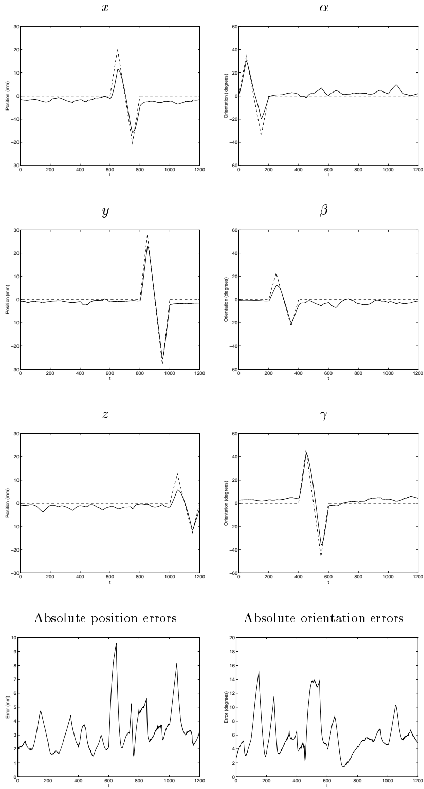
Figure 9: Commanded (dotted lines) and estimated (solid lines) positions and orientations, and estimated errors during a manipulation sequence.
