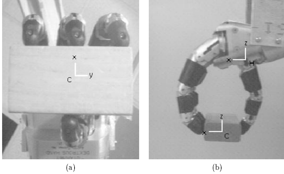
Figure 2: The hand-centered reference frame H and the object-centered reference frame C
