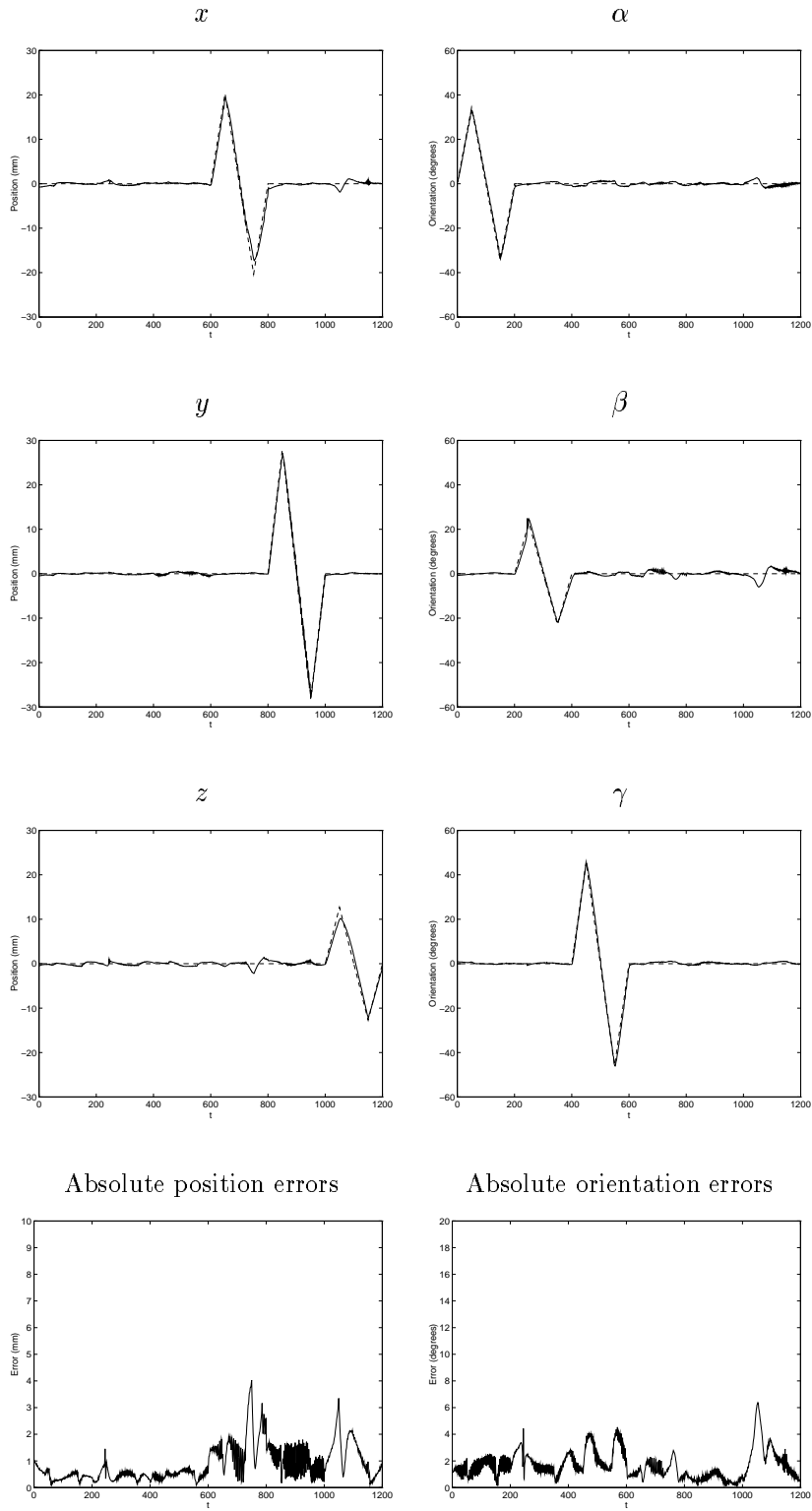
Figure 11: Commanded (dotted lines) and estimated (solid lines) positions and orientations, and estimated errors during a manipulation sequence.
