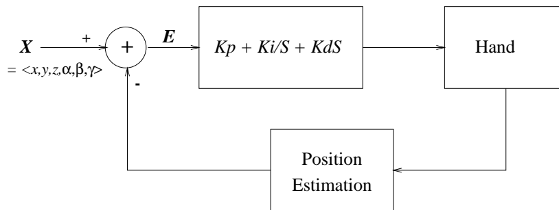
Figure 10: Control system
