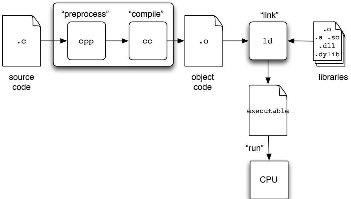
Figure 2: C Development and Execution Environment
