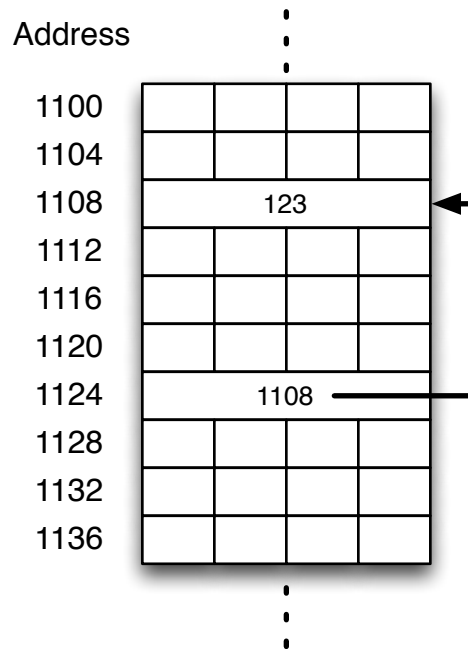
Figure 6: Variable and pointer in memory
