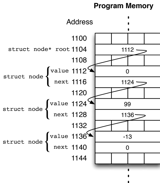
Figure 9: Dynamically allocated linked list
