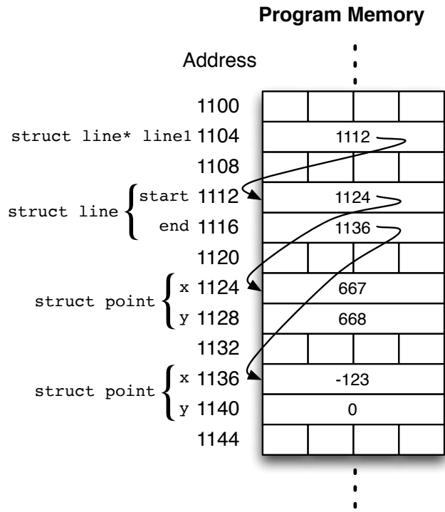
Figure 8: Dynamically allocated struct line with pointer members
