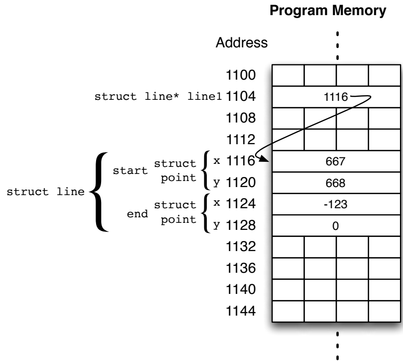
Figure 7: Dynamically allocated struct line
