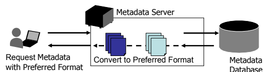
Figure 1: Metadata Conversion
