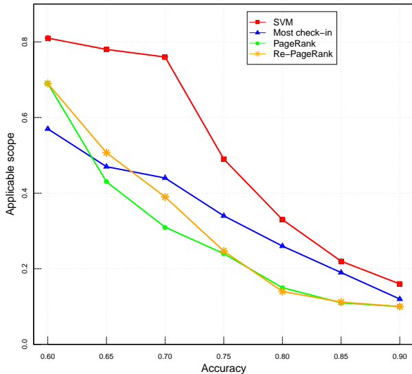
Figure 2: Comparison of our SVM method for home location prediction to prior approaches in New York City dataset, as coverage and accuracy vary.
