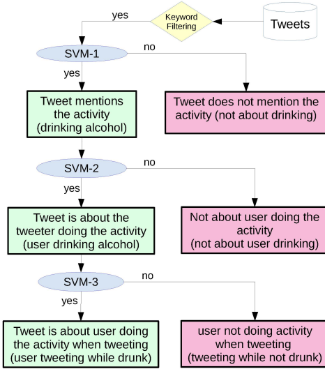
Figure 1: Flowchart for latent activity detection.
