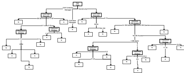
Figure 4: The full depiction tree for anomaly avoidance.
