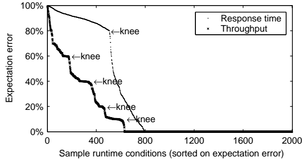
Figure 2: Response time and throughput expectation errors of 2000 sampled runtime conditions sorted in decreasing order. We mark knee points on the two curves for possible identification of the anomaly error threshold.
