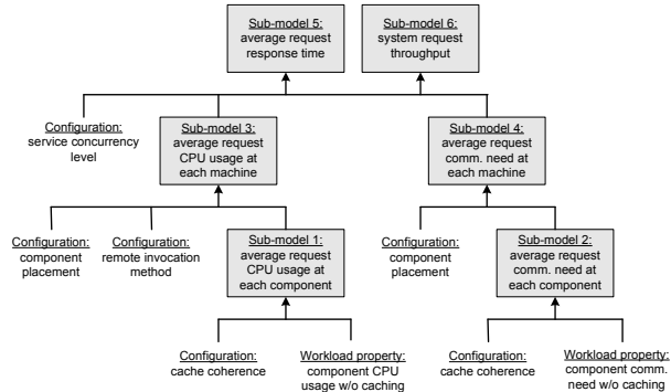
Figure 1: A hierarchy of sub-models. Low-level workload properties are assembled into higher-level properties according to the performance impact of configuration settings.
