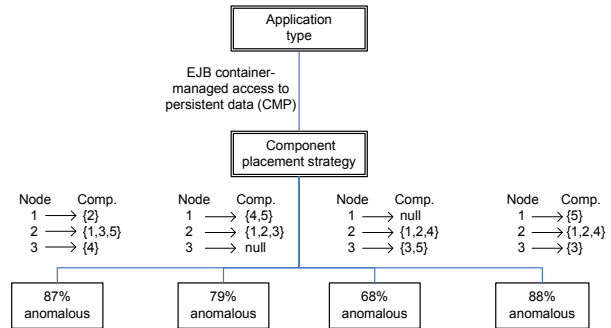
Figure 5: A three-level decision tree produced for debugging. Non-leaf nodes represent system configurations or workload conditions while leaf nodes represent decision points. The value inside each decision point indicates the likelihood of performance anomalies within that decision point's region. For brevity, we only show the decision points in the tree that are substantially anomalous.
