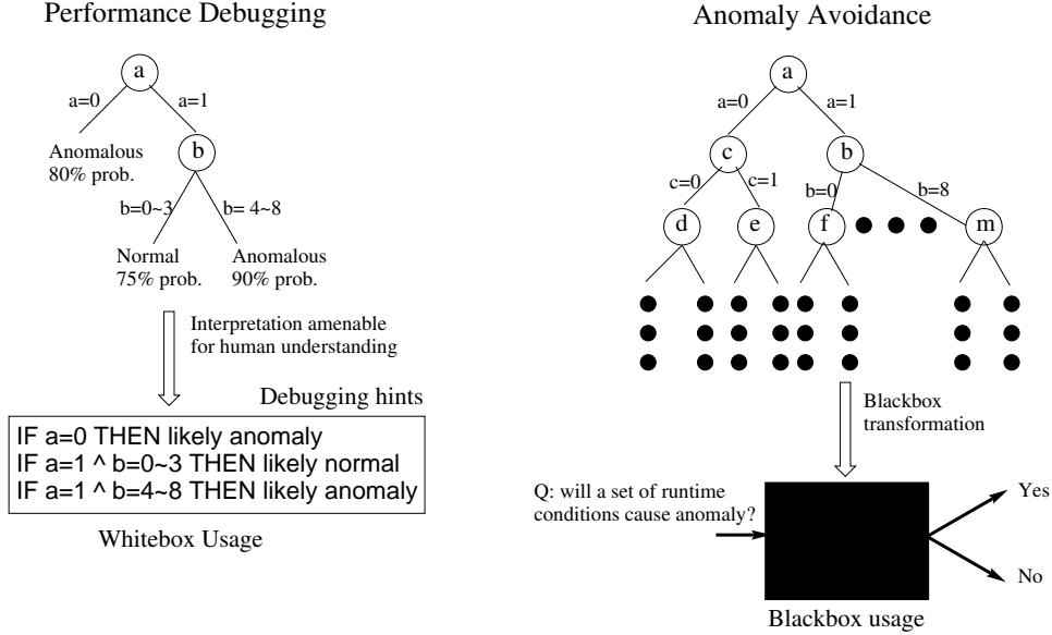
Figure 3: Decision tree-based performance anomaly depiction.
