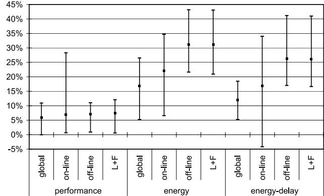
Figure 7. Minimum, maximum and average slowdown, energy savings, and energy \times delay improvement.
