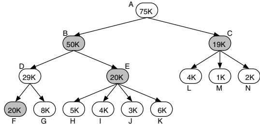
Figure 3. Call tree with associated instruction counts. The shaded nodes have been identified as candidates for reconfiguration.
