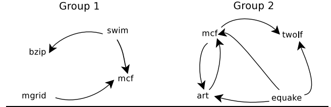
Figure 13. Contention relations of two groups of SPEC-CPU2000 benchmarks. If A points to B, that means B has more than 50% performance degradation when running together with A on a shared cache, compared to running alone when B can monopolize the whole cache.
