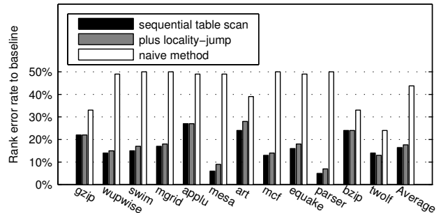
Figure 10. Rank error rate on identified page hotness between various approaches and the baseline (an approximation of “true page hotness”).
