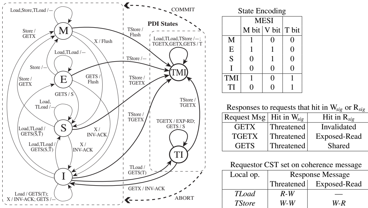
Figure 1: Dashed boxes enclose the MESI and PDI subsets of the state space. Notation on transitions is conventional: the part before the slash is the triggering message; after is the resulting action (‘-’ means none). GETS indicates a request for a valid sharable copy; GETX for an exclusive copy; TGETX for a copy that can be speculatively updated with TStore . X stands for the set {GETX, TGETX}. “Flush” indicates a data block response to the requestor and directory. S indicates a Shared message; T a Threatened message. Plain, they indicate a response by the local processor to the remote requestor; parenthesized, they indicate the message that accompanies the response to a request. An overbar means logically “not signaled”.
