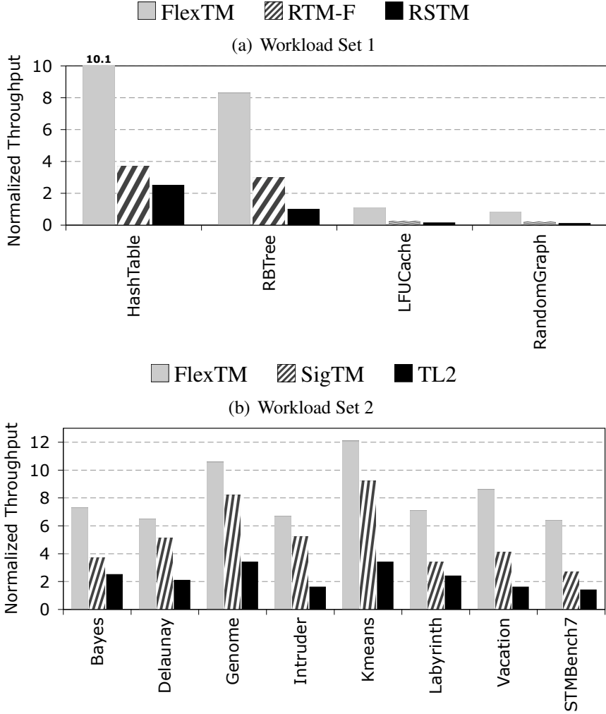
Figure 7: Throughput (transactions/ 10^6 cycles), normalized to sequential thread. All performance bars use 16 threads.
