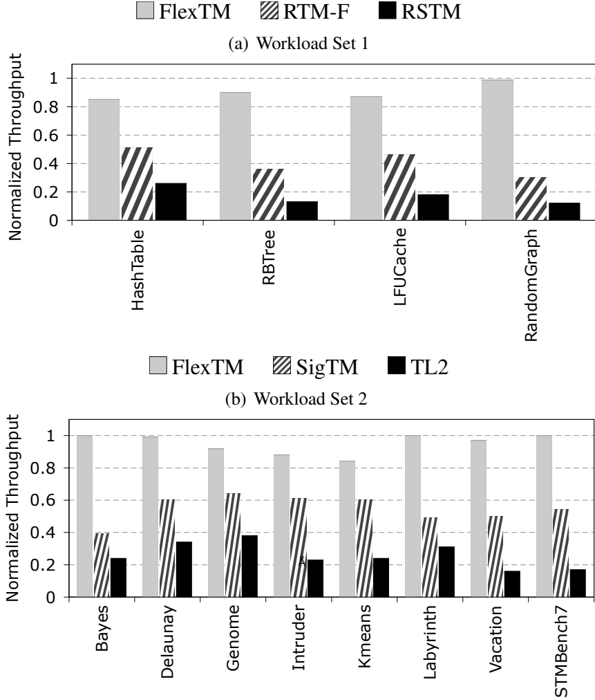
Figure 6: Throughput (transactions/ 10^6 cycles), normalized to sequential thread. All performance bars use 1 thread.
