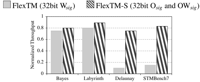
Figure 10: Signature size effect (relative to FlexTM with 2048-bit W_{sig} ).
