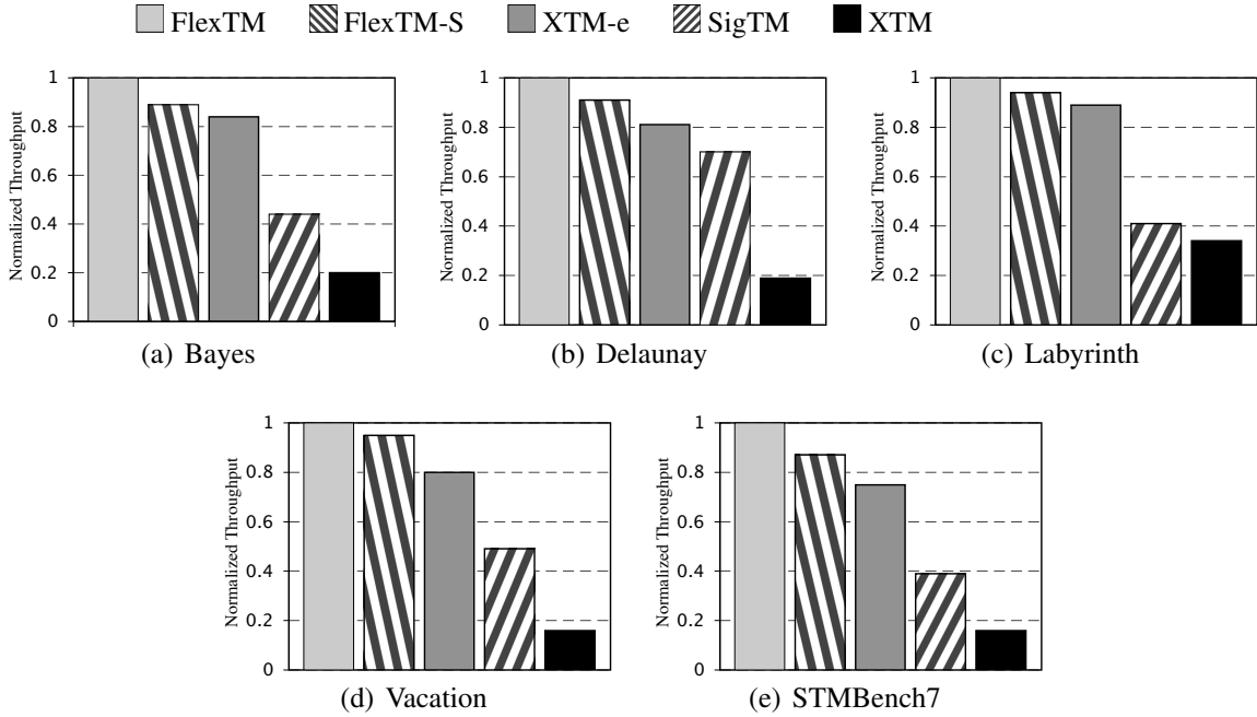
Figure 9: Throughput at 16 threads for FlexTM-S vs. other TMs, normalized to FlexTM.
