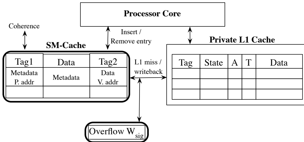
Figure 5: Simplified overflow support with SM-cache. Dashed lines surround new extension that replaces the OT controller (see Figure 2).
