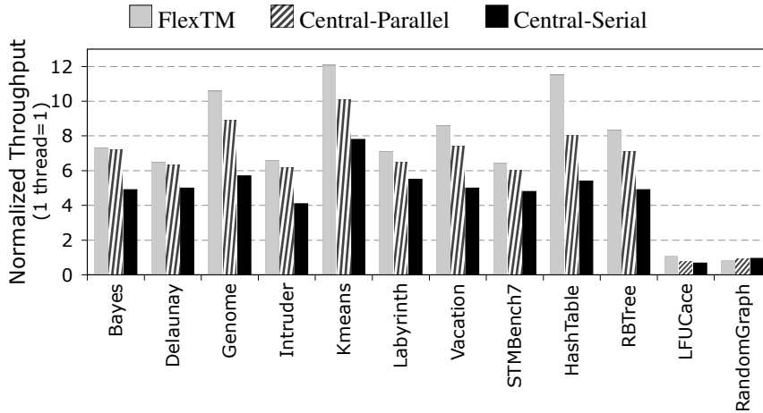
Figure 8: FlexTM vs. Centralized hardware arbiters.
