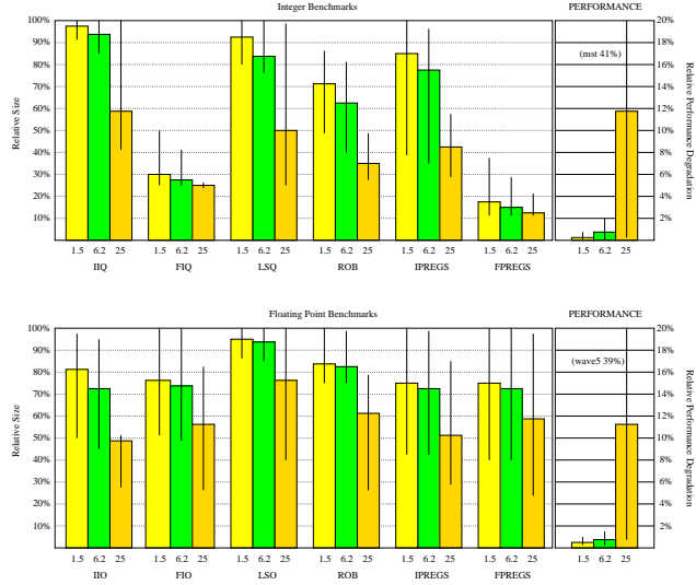
Figure 5. Buffer Relative Sizing and Performance
