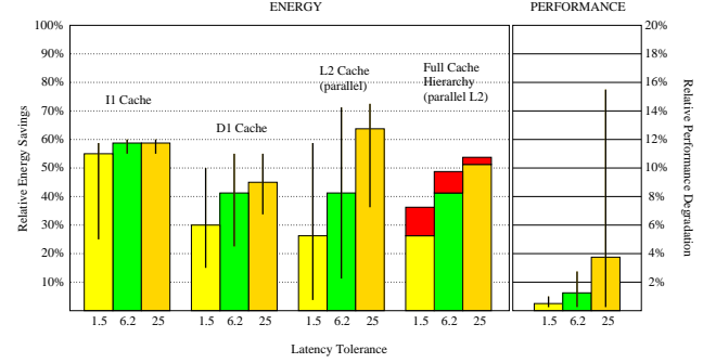
Figure 4. Relative cache energy usage averaged across all benchmarks
