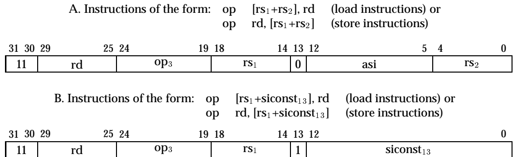
Figure 9.1 Instruction formats for load and store instructions
