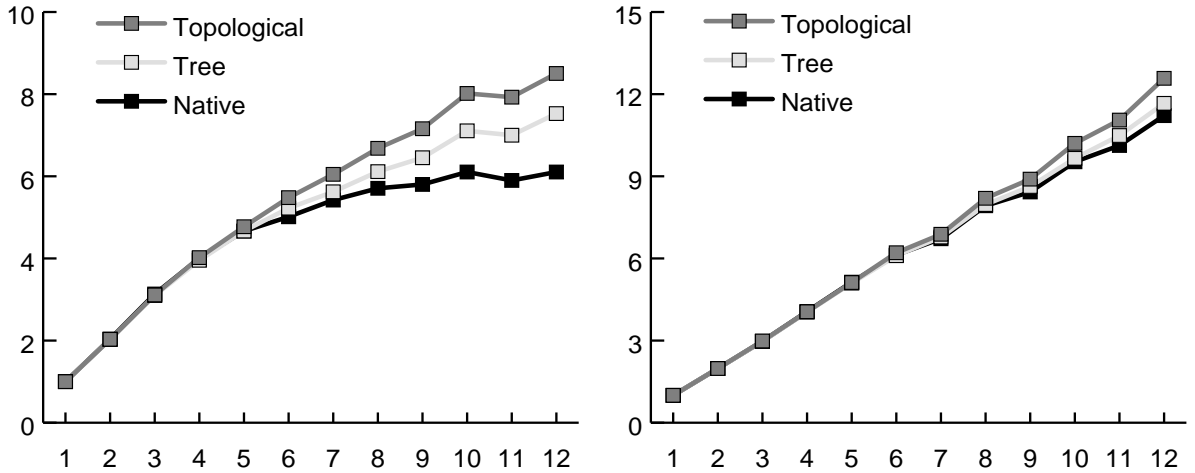
Figure 4: Speedup graphs for SOR (left) and Mgrid (right) on a 12-processor SGI Challenge. Absolute times on one processor are the same for all three barriers.
