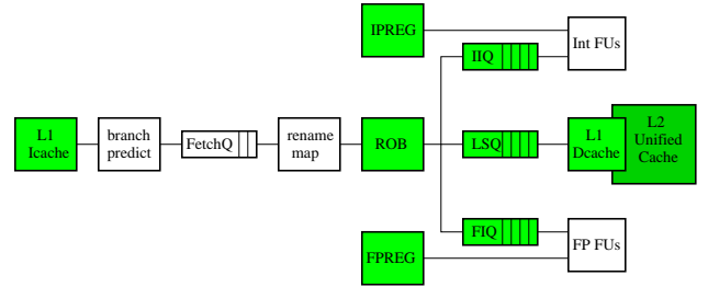
Figure 1. The Base Microarchitecture: Adaptable components are shaded
