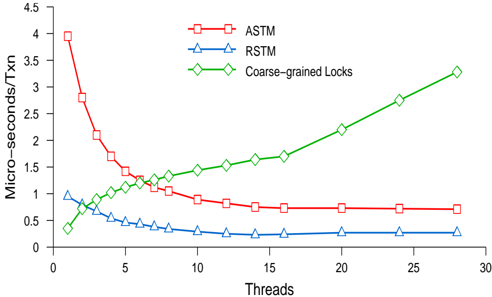
Figure 2: Performance scaling of RSTM, ASTM, and coarse-grain locking on a hash table microbenchmark.
