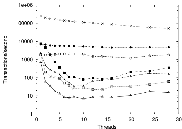
Figure 8. RandomGraph.
