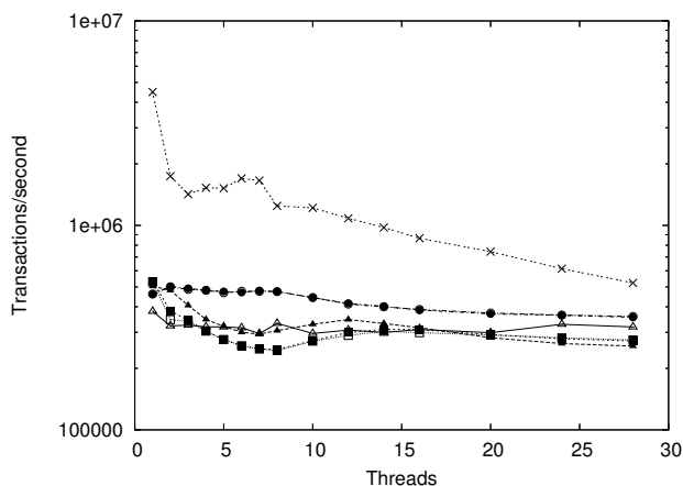
Figure 9. LFUCache.
