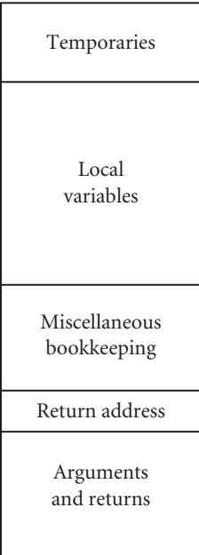
Subroutine 1
