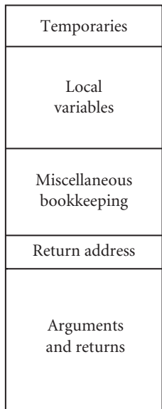
Subroutine 3
