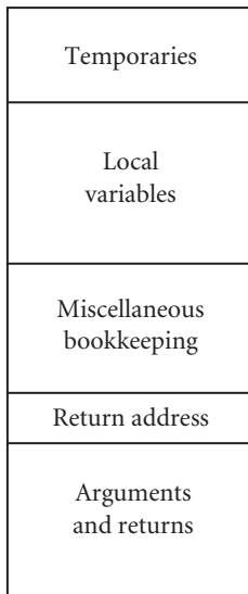
Subroutine 2
