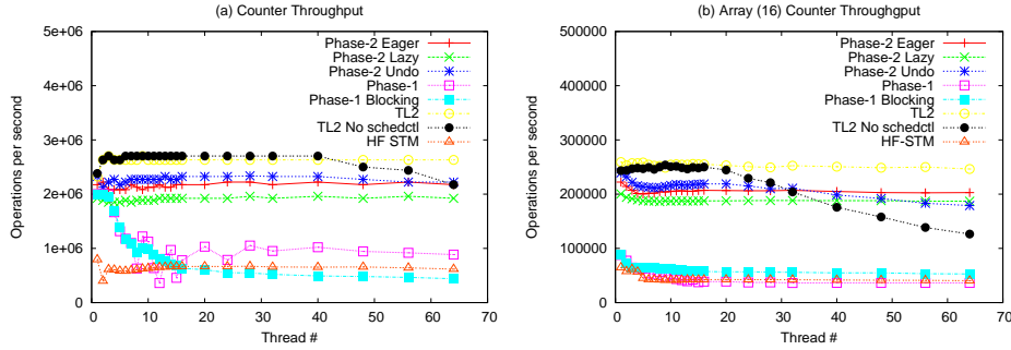
Figure 7. Throughput on the shared Counter (cntnr) and Array of 16 Counters (array_cntnr) benchmarks.
