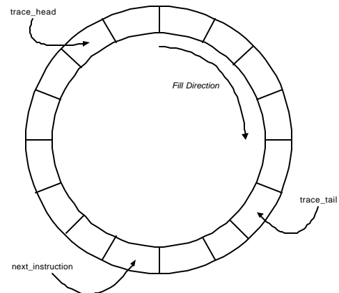
Figure 3: The Sliding Window Fill Mechanism
