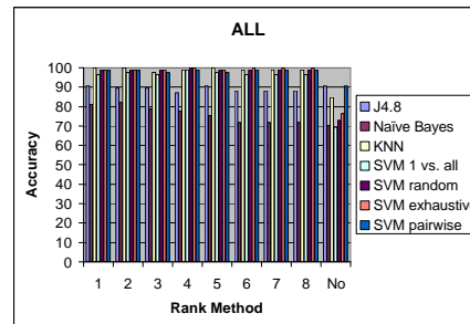
Figure 3: ALL Dataset
