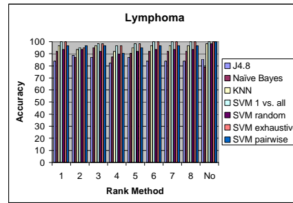
Figure 7: Lymphoma Dataset
