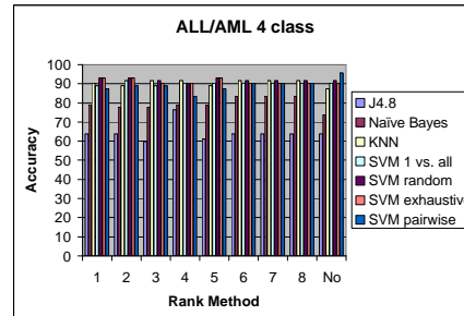
Figure 2: ALLAML4 Dataset
