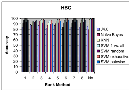
Figure 9: HBC Dataset
