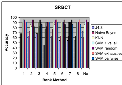
Figure 5: SRBCT Dataset
