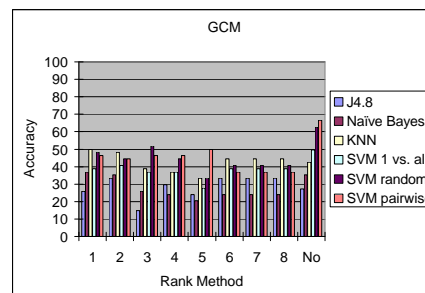
Figure 4: GCM Dataset
