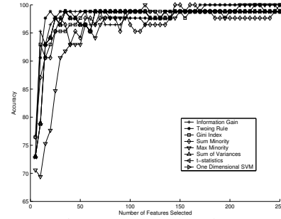
Figure 1: SVM Random
