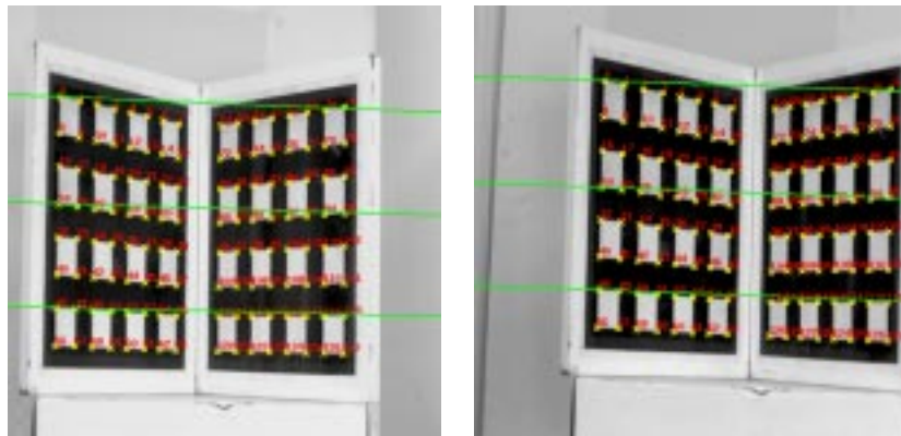
Figure 2. A two-plane model used in the classical calibration technique.
