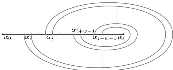
Fig. 1 A block of 4-cells \alpha[i:i + w - 1] reattaching to \alpha on the opposite side in \alpha[j:j + w - 1] overlapping the original block \alpha[i:i + w - 1] in \alpha[j:i + w - 1]
