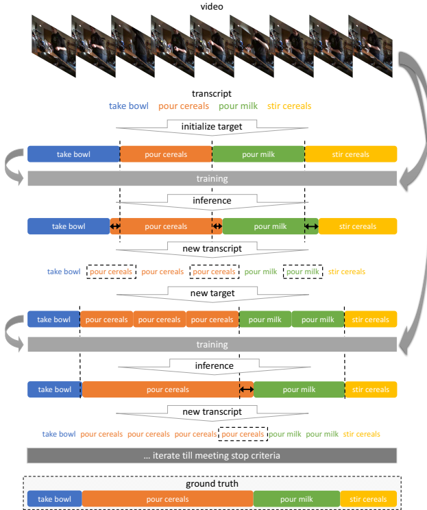
Figure 4. Overview of the proposed Iterative Soft Boundary Assignment (ISBA) strategy. Under weak supervision, we start from the action transcript and initialize the training target by uniform mapping. A temporal segmentation model is then trained and with which we infer the result on the training set. The action transcript is then refined by the training result and the next iteration starts. Finally until meeting the stop criteria, the final model is used to infer on the training set for the alignment task, and predict on the testing set for the segmentation task.
