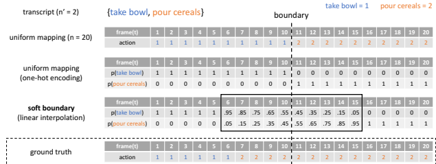
Figure 3. Example case of the proposed soft boundary mechanism. By using linear interpolation of probabilities, the temporal boundary between two different actions becomes coarse, which makes the generated target more robust and reliable.
