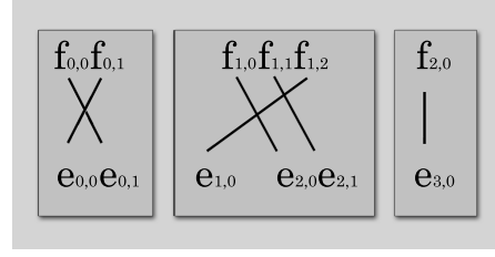
Figure 3: Morpheme alignment
