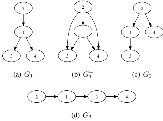
Figure 1: Scoping as DAG
