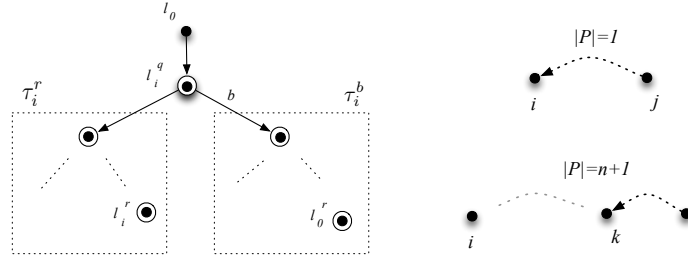
Figure 20: Proof of Theorem 17 ( l_k^r represents an arbitrary node in T_k^r ).
