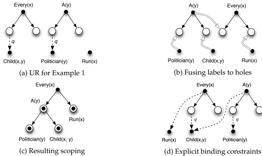
Figure 2: Using graphical notation to represent unscoped LF
