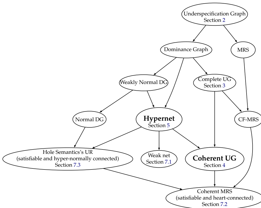
Figure 1: Classes of Underspecification Graph introduced in this article. We define Hypernet, show that it is computationally tractable, and further show that it covers all coherent sentences, and that it subsumes previously identified tractable classes.
