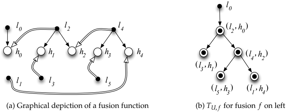
Figure 4: Building a solution for a UG
