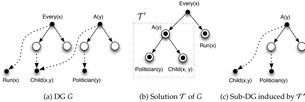
Figure 11: DG counterpart of the UG for Every child of a politician runs and a sub-DG of it
