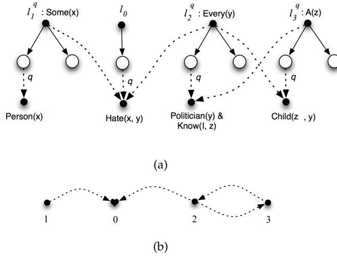
Figure 10: UG and SDG for Somebody hates every politician whom I know a child of
