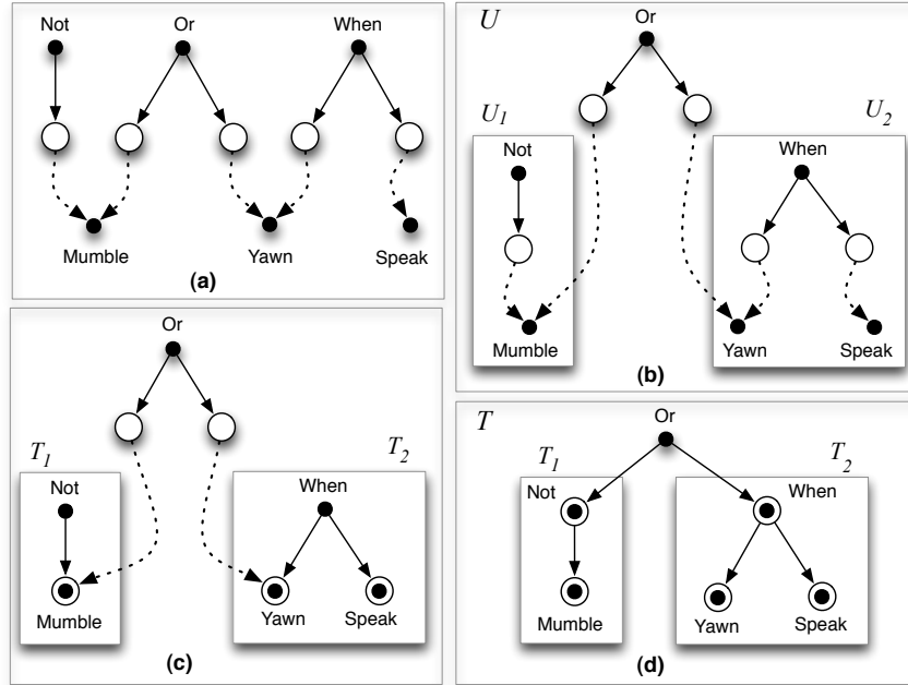
Figure 12: Recursive construction of solutions
