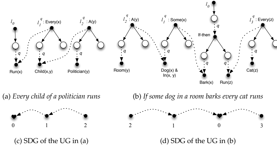
Figure 9: Constructing semantic dependency graph
