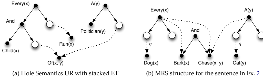
Figure 5: Examples of stacked ETs
