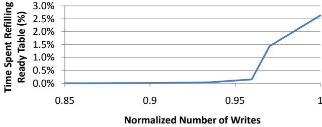
Figure 8. Expected percentage of total CPU time consumed by refilling the ready table as a function of device age.
