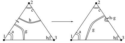
Fig. 4. Pulling the curve to a normal position (w.l.o.g. h \geq g ).
