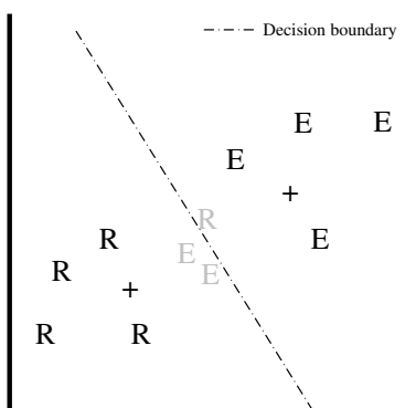
Figure 2: Plausible centroids
