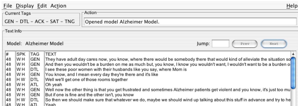
Figure 10: CATS tags data and gives a certainty measure to its left. Low certainty tags can be glanced over by the researcher to assure correctness.
