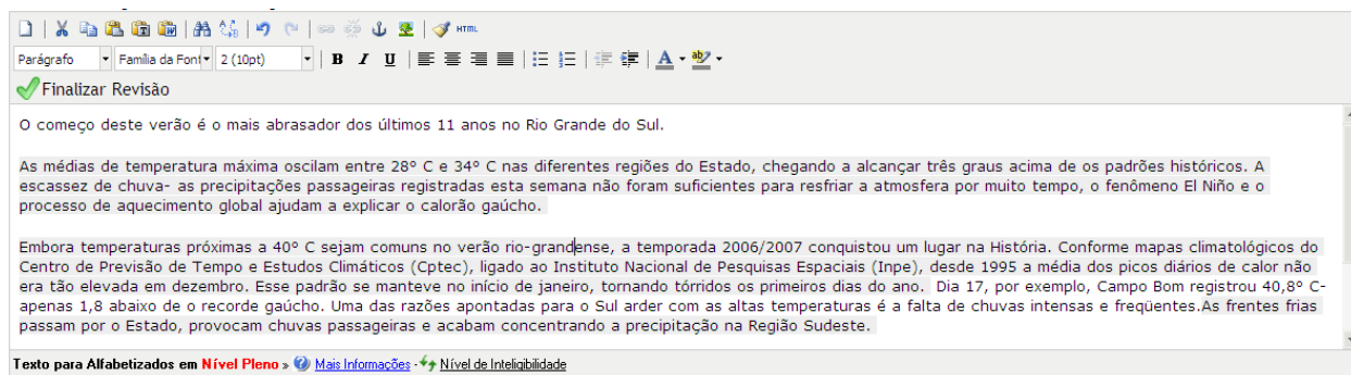
Figure 1: SIMPLIFICA interface
