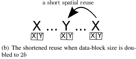
Figure 2. Example spatial reuse. Data X and Y have size b and reside in the same 2b block. When the data-block size is 2b , the original reuse in Part (a) is shortened by an intercept as shown in Part (b).
