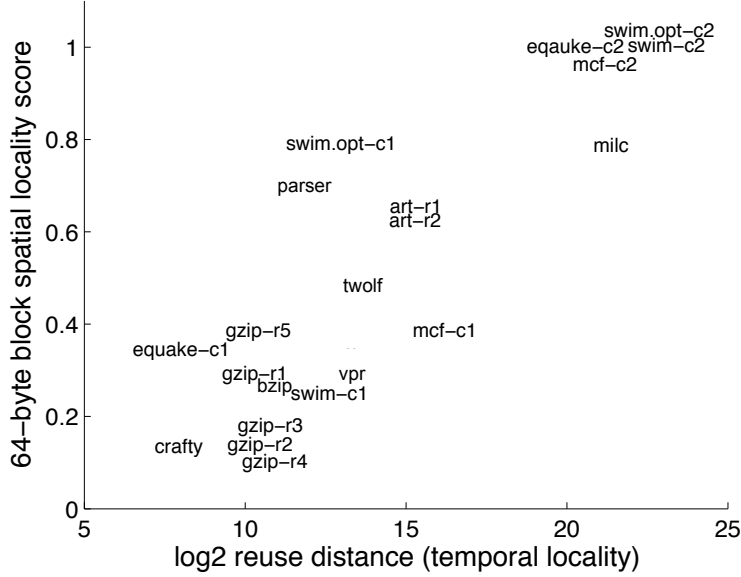
Figure 3. The spatial and temporal locality of spatial locality components. The y -axis shows the spatial-locality score, the higher the better. The score of one means perfect spatial locality. The x -axis shows the reuse distance in a logarithmic scale. The further to the right, the poorer is the temporal locality. Data layout transformations are most cost effective when targeted for components on the bottom-right half of the plot, which have poor spatial and temporal locality.
