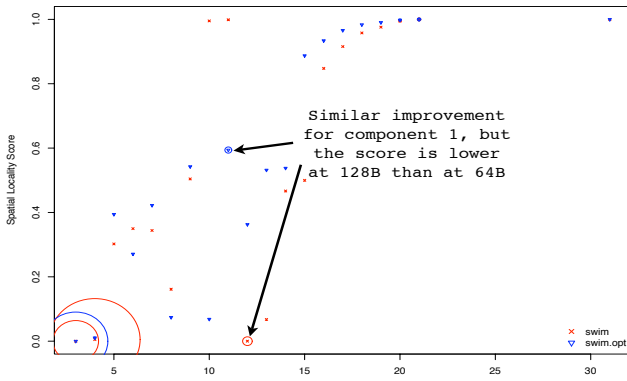
Figure 6. The effect of array regrouping on adjacent-block spatial locality, measured by the spatial-locality score when the measurement block size increases from 64 bytes to 128 bytes.
