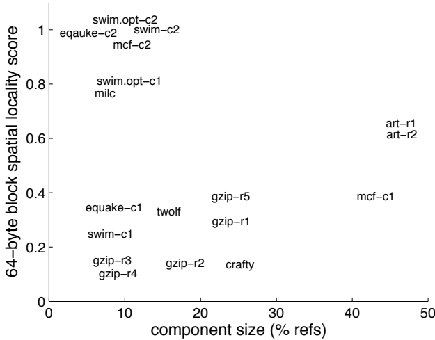
Figure 4. The size of spatial-locality components shown in Figure 3
