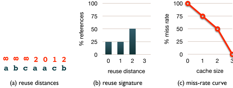
Figure 1. Example reuse distances, reuse signature, and miss-rate curve
