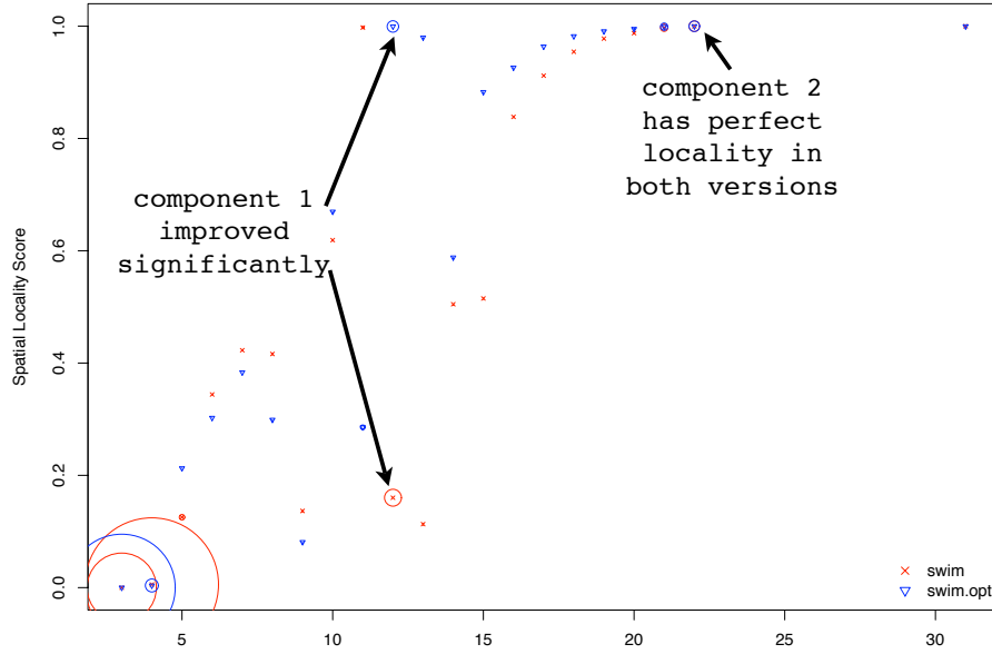
Figure 5. The effect of array regrouping on the spatial-locality score of each reuse-distance bin of Swim . The improvement comes mainly from better spatial locality for the first component.
