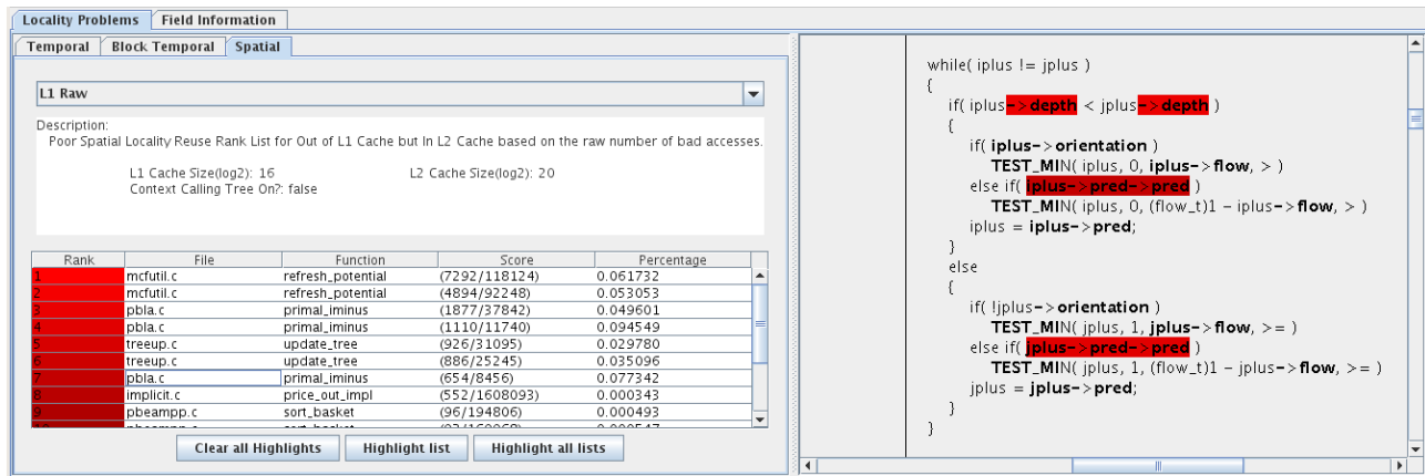
Figure 7. The GUI interface of the new analysis displaying the spatial-locality ranking of program code. The list of ten program statements in Mcf that contribute most to the poor spatial locality are shown in the left half of the screen shot. A user can view these statements in program code, as shown in the right half of the screen shot.
