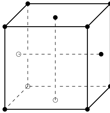
Figure 4.20: A counterexample demonstrating that the three-dimensional Delaunay refinement algorithm is not size-optimal.
