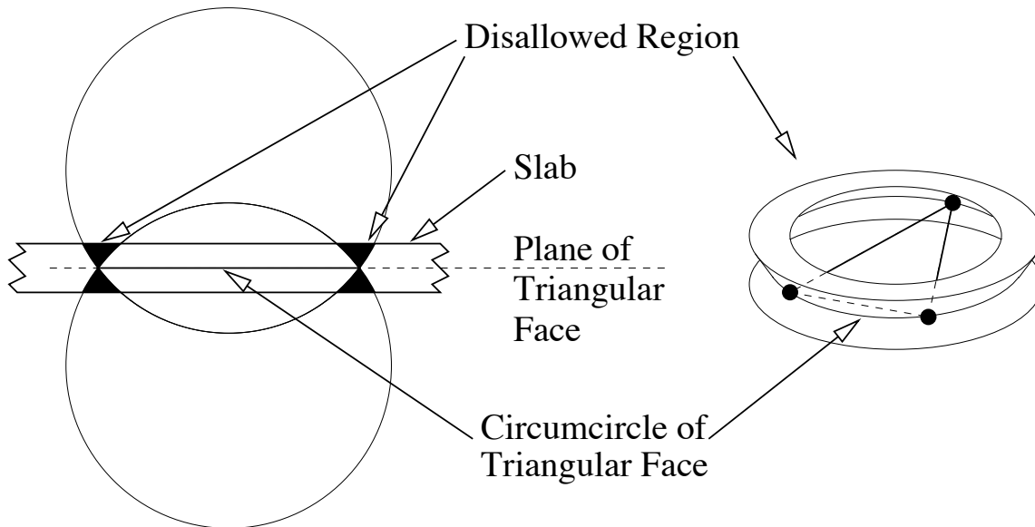
Figure 4.23: Left: A side view of the plane containing a triangular face. In conjunction with this face, a newly inserted vertex can form a sliver with both a bad dihedral angle and a good circumradius-to-shortest edge ratio only if it is inserted in the disallowed region (black). Right: An oblique view of the disallowed region of a triangular face.
