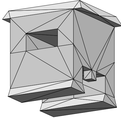
Initial tetrahedralization after segment and facet recovery. 71 vertices, 146 tetrahedra.
