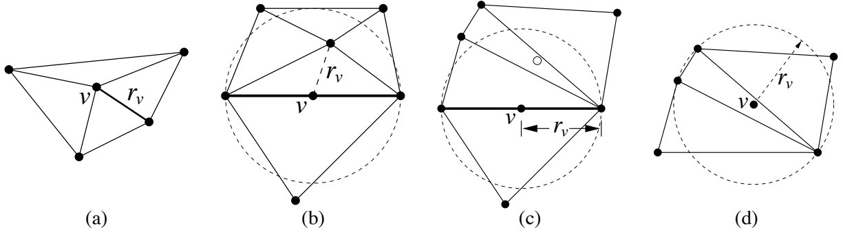
Figure 3.14: The insertion radius of a vertex v is the distance to the nearest vertex when v first appears in the mesh. (a) If v is an input vertex, r_v is the distance to the nearest other input vertex. (b) If v is the midpoint of a subsegment encroached upon by a mesh vertex, r_v is the distance to that vertex. (c) If v is the midpoint of a subsegment encroached upon only by a rejected vertex, r_v is the radius of the subsegment's diametral circle. (d) If v is the circumcenter of a skinny triangle, r_v is the radius of the circumcircle.
