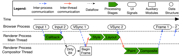
Fig. 7: The simplified view of frame lifetime in modern multi-process/thread browsers. A frame starts when the browser process receives an input event and ends when the frame is displayed and the browser process is signaled. In between, an input event is processed by different stages spread across multiple threads. Different input events might interleave with each other.
