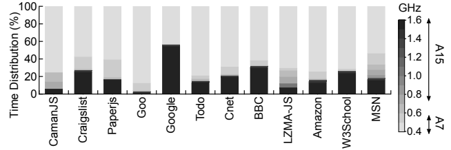
(b) Architecture configuration distribution for GreenWeb-U .
