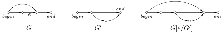
Figure 2.1: The replacement of an edge.
