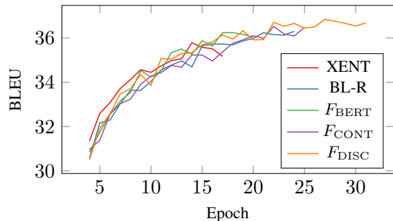
Figure 1: Development set BLEU during fine-tuning.
