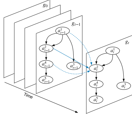
Figure 3: Architecture of the graph recurrent network.
