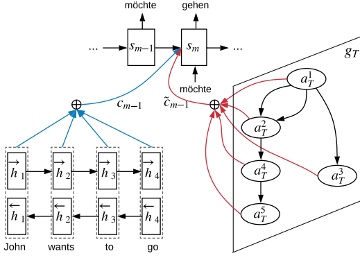
Figure 2: Overall architecture of our model.
