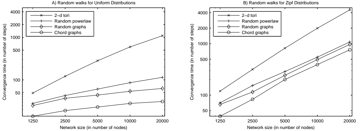
Fig. 2. Random walk convergence time on different network sizes, topologies and node visitation distributions. We use topologies with an average node degree of 4. In the simulation, the random powerlaw graph is generated by linking each new node to existing nodes chosen randomly with probability proportional to their degrees. Such a preferential link creation process is known to generate topologies with powerlaw degree distributions [5], [9]. We generate random graphs by a simple process of linking each node to some other nodes chosen uniformly at random.
