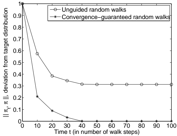
Fig. 5. The convergence of random walk node visitation probability distribution on random powerlaw graphs (20000 nodes).
