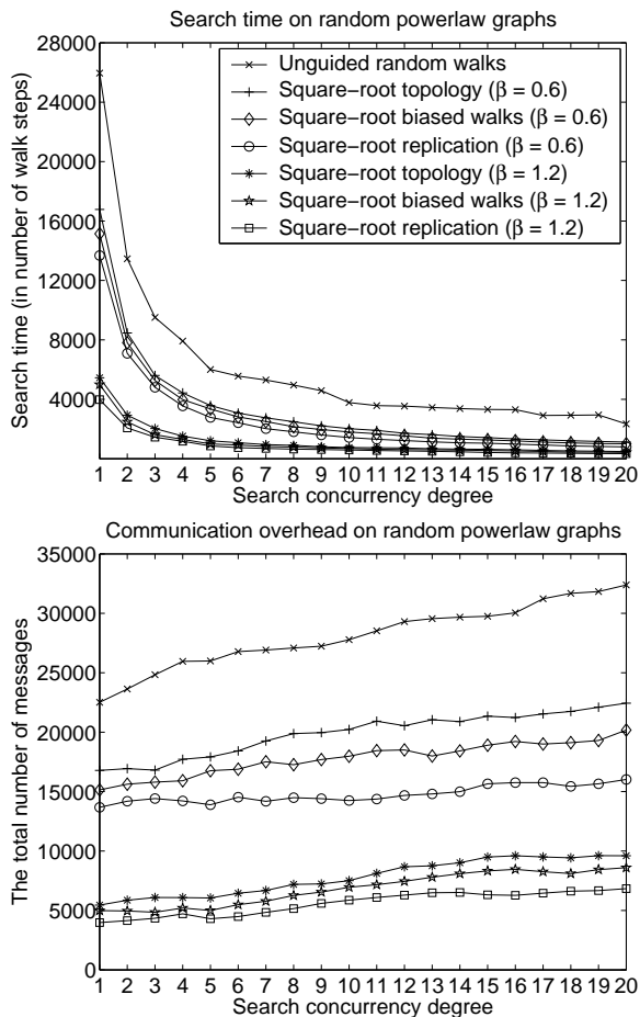
Fig. 7. The search time and communication overhead on random powerlaw graphs (20000 nodes). The search concurrency degree represents the number of random walkers (or the average number of replication copies for square-root replication).
