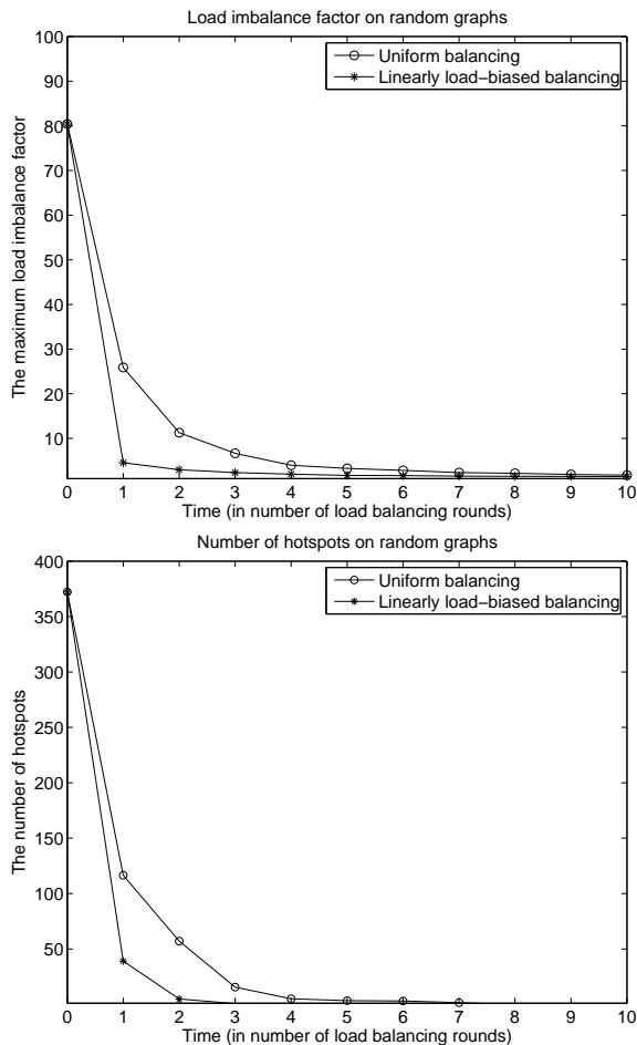
Fig. 8. The maximum load imbalance factor and the number of hotspots on random graphs (20000 nodes).
