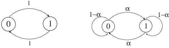
Fig. 1. An illustration on how self-loops achieve unique convergence of random walks.
