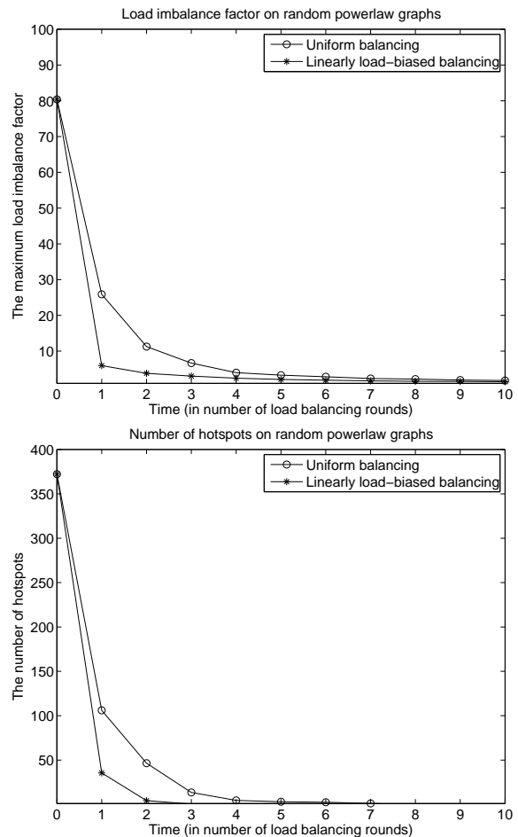
Fig. 9. The maximum load imbalance factor and the number of hotspots on random powerlaw graphs (20000 nodes).
