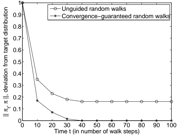
Fig. 4. The convergence of random walk node visitation probability distribution on random graphs (20000 nodes).
