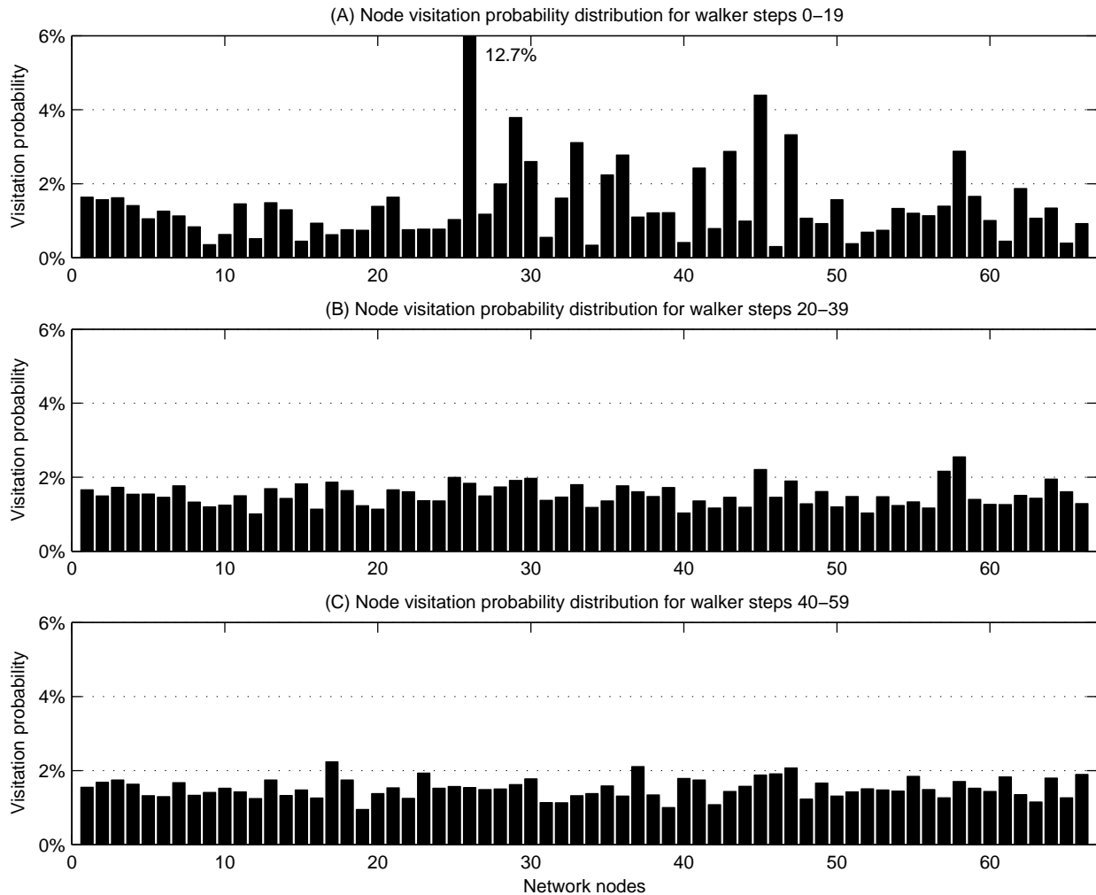
Fig. 11. Node visitation probability distributions of convergence-guaranteed random walks on a random topology with 66 Planetlab nodes. The converged distribution is the uniform distribution.
