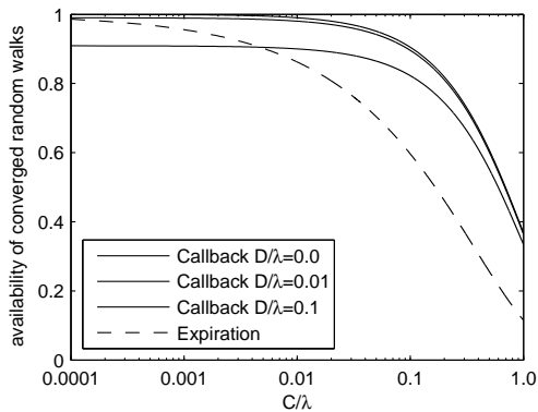
Fig. 3. The availability of two walker loss recovery methods when walker may be lost due to node failures. Note that the X-axis is in the logarithmic scale. We assume nodes fail independently of each other and we also assume each network node follows a memory-less failure model with an exponential distribution for the time to next failure. \lambda represents MTTF of node failures. C represents the convergence time for a newly initiated random walk. For the Callback method, we show three availability curves with D/\lambda = 0.0 , D/\lambda = 0.01 , and D/\lambda = 0.1 respectively (where D represents the walker loss detection delay). A curve with a smaller D is higher in the figure.
