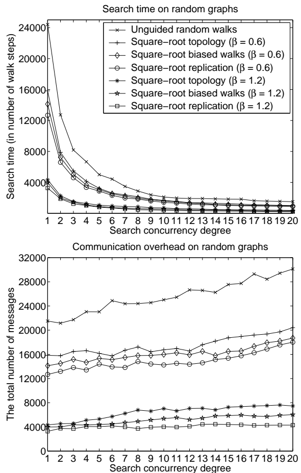
Fig. 6. The search time and communication overhead on random graphs (20000 nodes). The search concurrency degree represents the number of random walkers (or the average number of replication copies for square-root replication).
