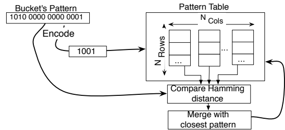
Fig. 7: Inserting and merging a pattern into the pattern table.
