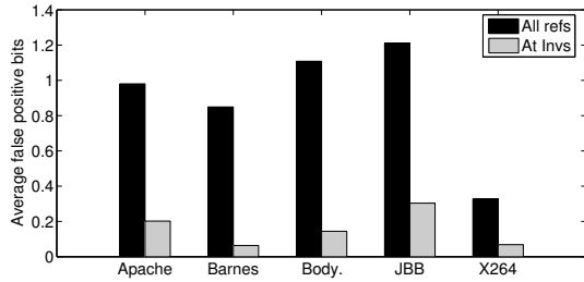
Fig. 10: False sharers on coherence write invalidations.
