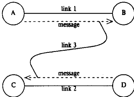
figure 1: link moving at both ends
