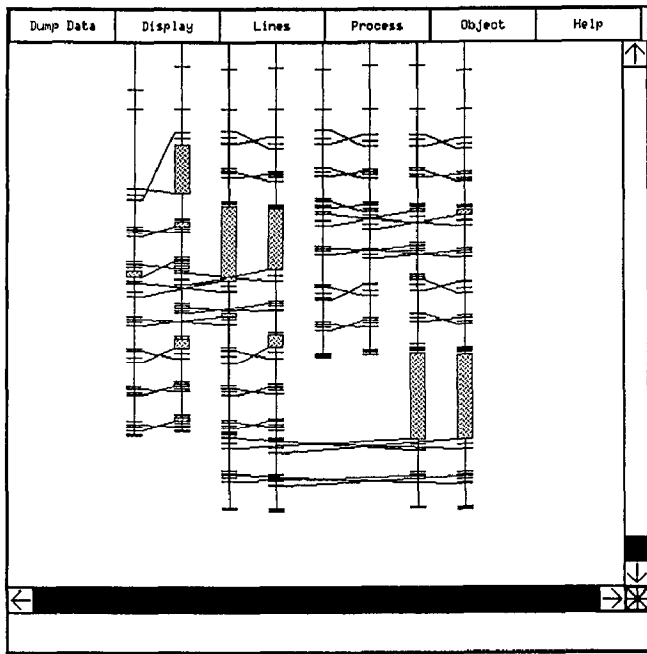
Figure 6: Graphical View of Odd-Even Merge Sort
