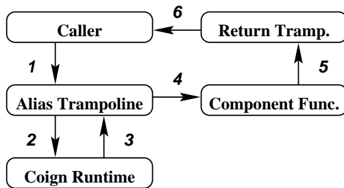
Figure 4: Calling sequence for first call to an aliased function without IDL information. Control passes from caller to trampoline function (1) then into the Coign runtime (2). The runtime returns a special value to the trampoline (3) which patches the stack. Control jumps directly into the component function (4) which returns to another trampoline (5) and then jumps back into the caller (6).
