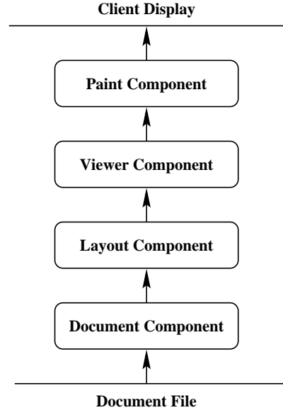
Figure 7: Simplified composition of the word-processing components.
