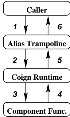
Figure 3: Calling sequence for an aliased function. Control passes from caller to trampoline function (1), through the Coign runtime (2) into the component (3) and back (4,5,6).
