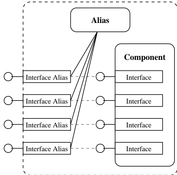
Figure 2: A component and its alias. The component alias creates an interface alias for each real interface.
