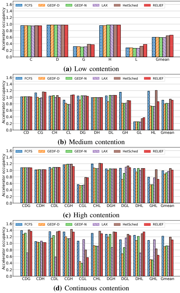
Fig. 7: Accelerator occupancy is defined as ratio of the sum of total of all accelerators’ compute time to the end-to-end system execution time, measured from the initiation of all applications to the completion of the last application. Higher is better.
