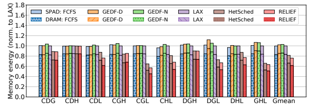
Fig. 6: Total main memory and scratchpad memories’ energy consumption under high contention using gem5-SALAM’s energy models.
