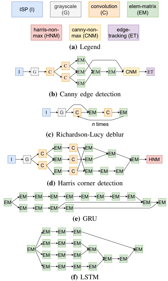
Fig. 1: Kernels in different image processing and RNN applications
