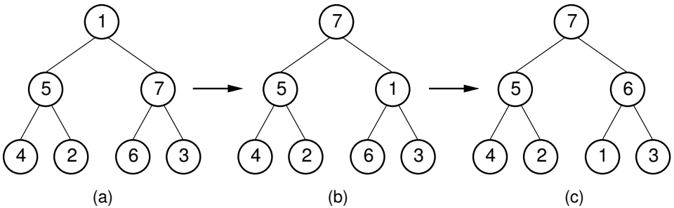
Figure 5.22 The siftdown operation. The subtrees of the root are assumed to be heaps. (a) The partially completed heap. (b) Values 1 and 7 are swapped. (c) Values 1 and 6 are swapped to form the final heap.
