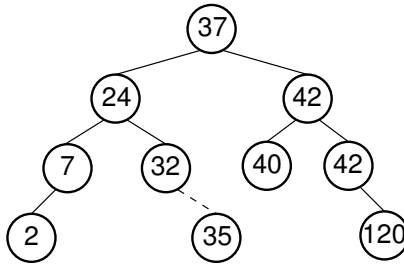
Figure 5.15 An example of BST insertion. A record with value 35 is inserted into the BST of Figure 5.13(a). The node with value 32 becomes the parent of the new node containing 35.
