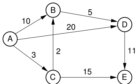
Figure 11.16 Example graph for shortest-path definitions.
