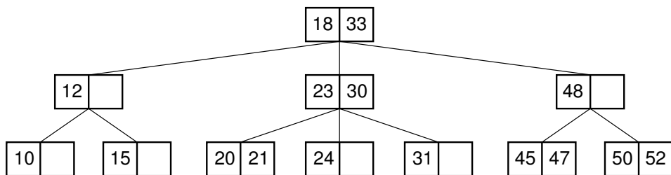
Figure 10.9 A 2-3 tree.
