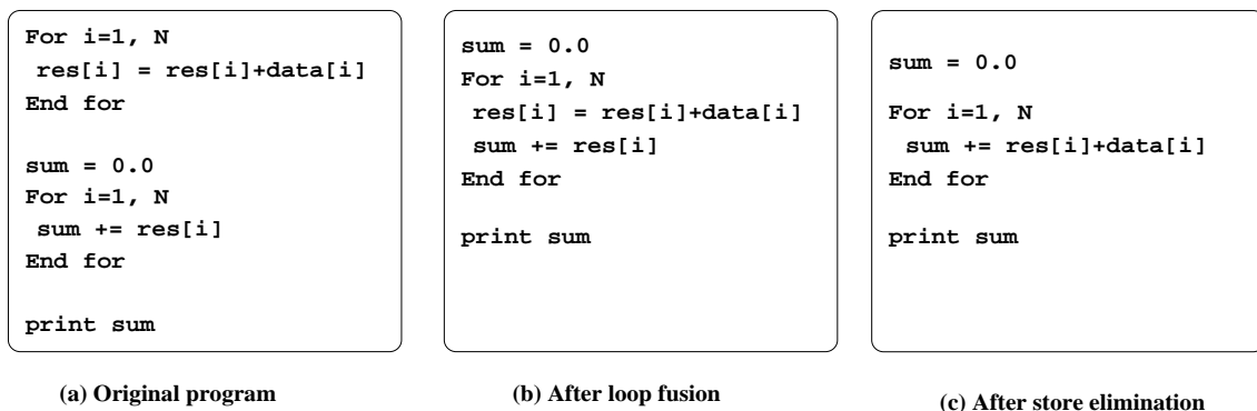
Figure 2.12 Store elimination
