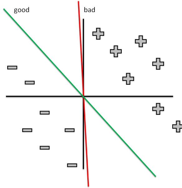
Figure 1: Linear Separability
