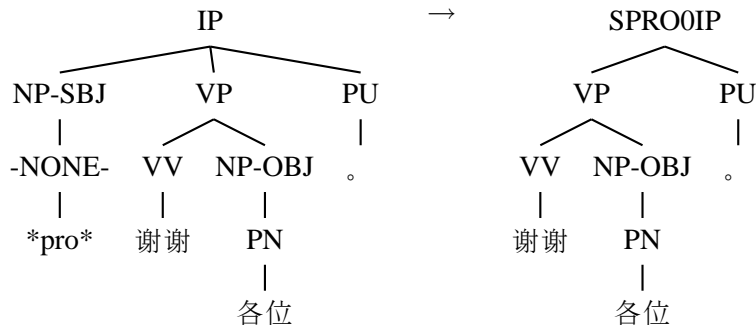
Figure 2: An example of tree modification
