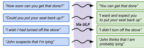
Figure 1: Examples of the sorts of discourse inferences that we generate via ULFs.
