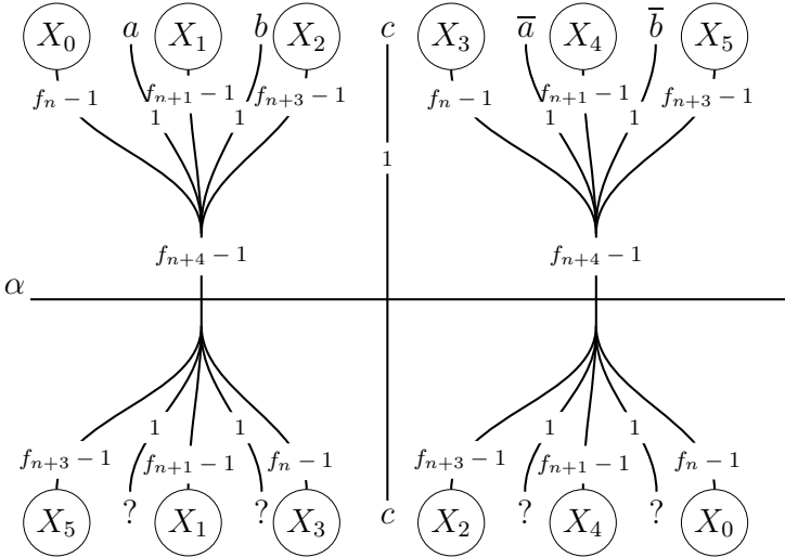
Fig. 1. Intersection of \alpha with a system of curves containing no spirals.
