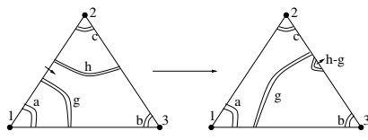
Fig. 4. Pulling the curve to a normal position (w.l.o.g. h \geq g ).
