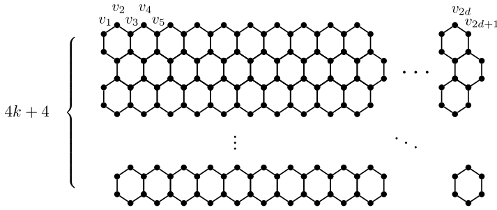
Fig. 3 Hexagonal grid replacing vertex
