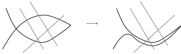
Fig. 6 Removing a minimal bigon and a crossing; changing the rotation
